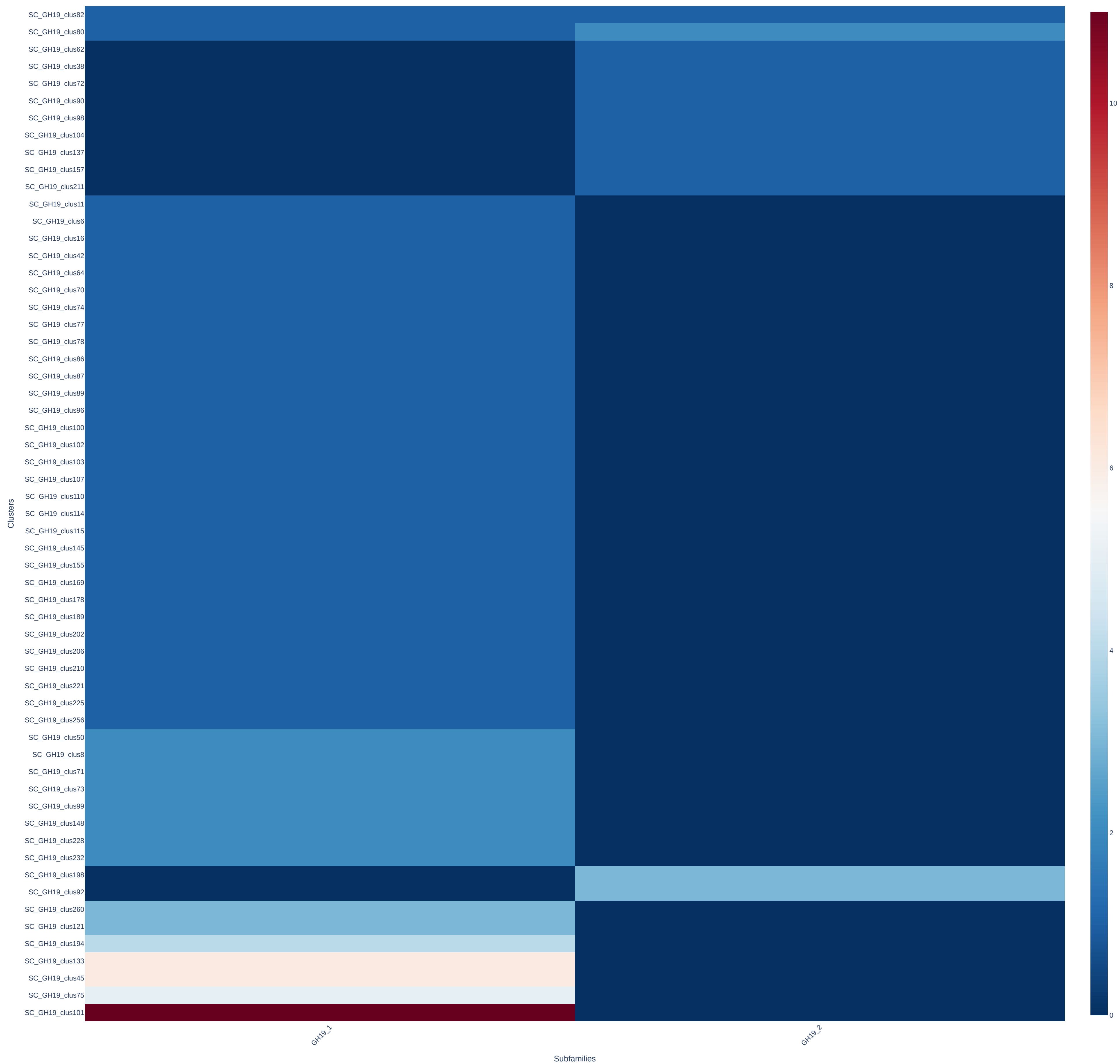
Interactive Heatmap for Family: GH19
