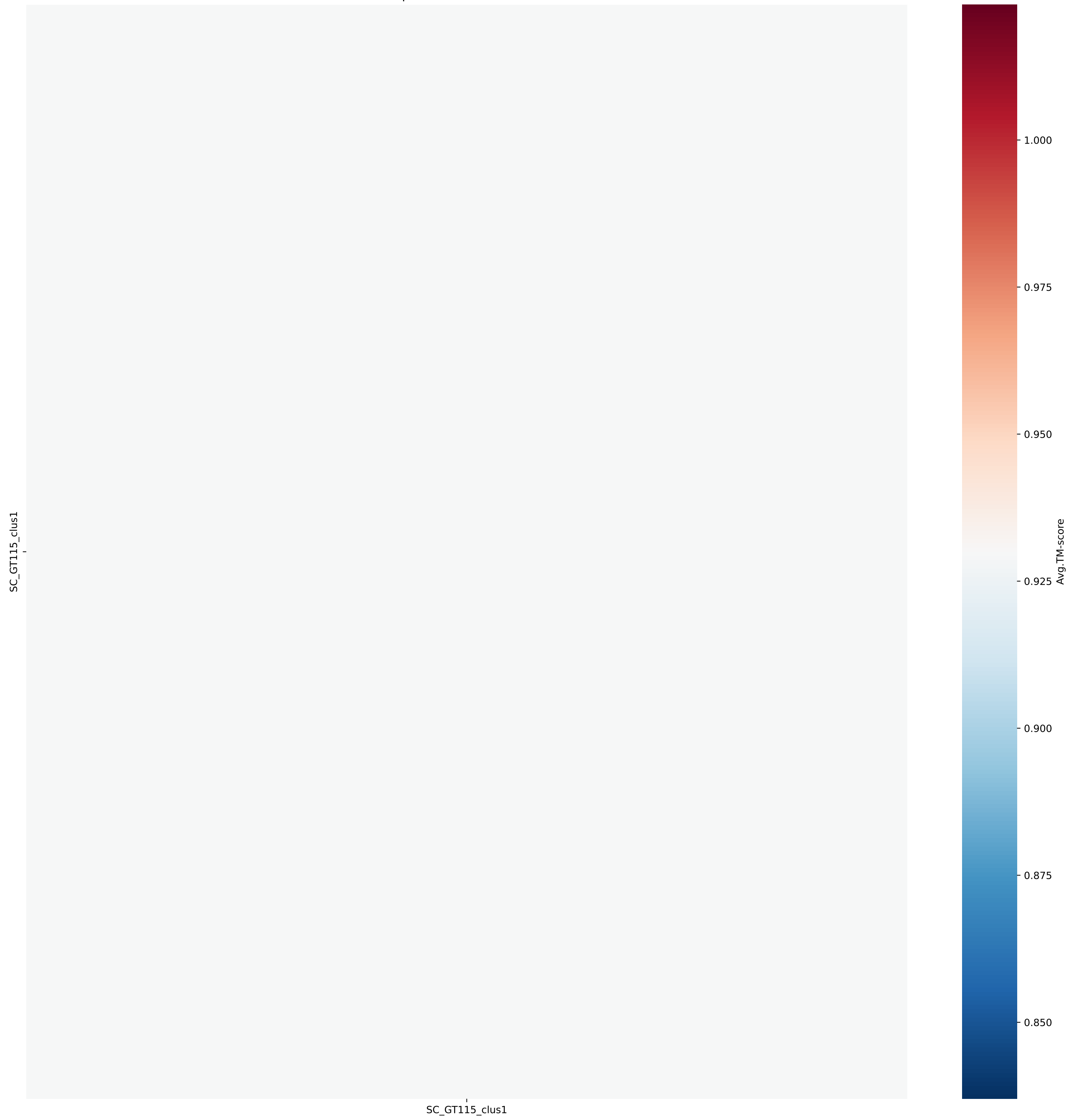
Heatmap of GT115 structural clusters
