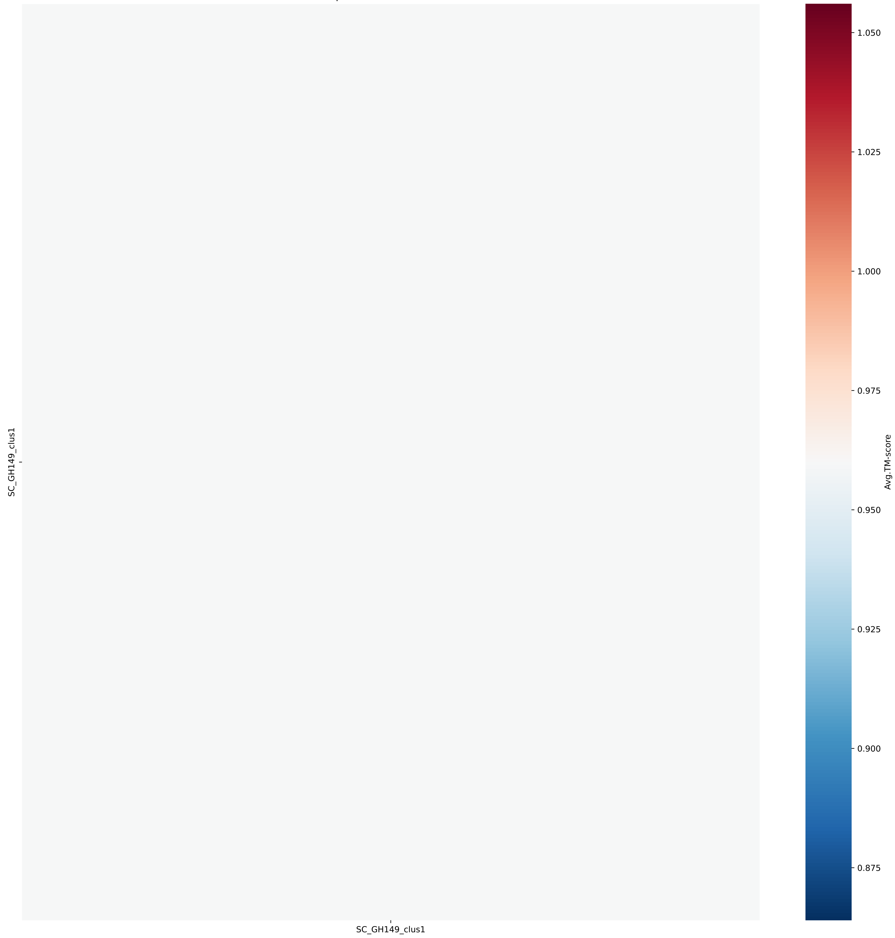
Heatmap of GH149 structural clusters
